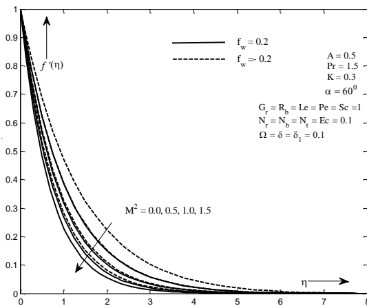
Fig. 3 Influence of M^2 on velocity profile
