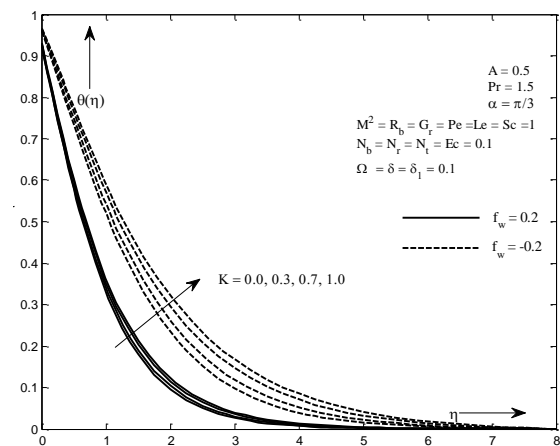
Fig. 13 Influence of K on temperature profile
