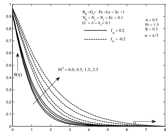
Fig. 12 Influence of M^2 on temperature profile
