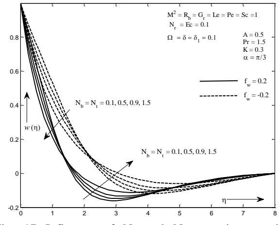
Fig. 17 Influence of N_b and N_t on microorganism conservation profile
